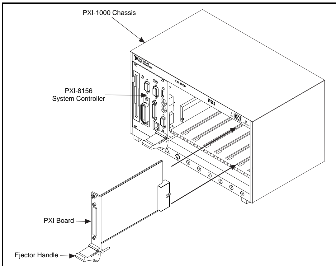
Figure 3-2. Installing the PXI-8320 in a PXI Chassis
