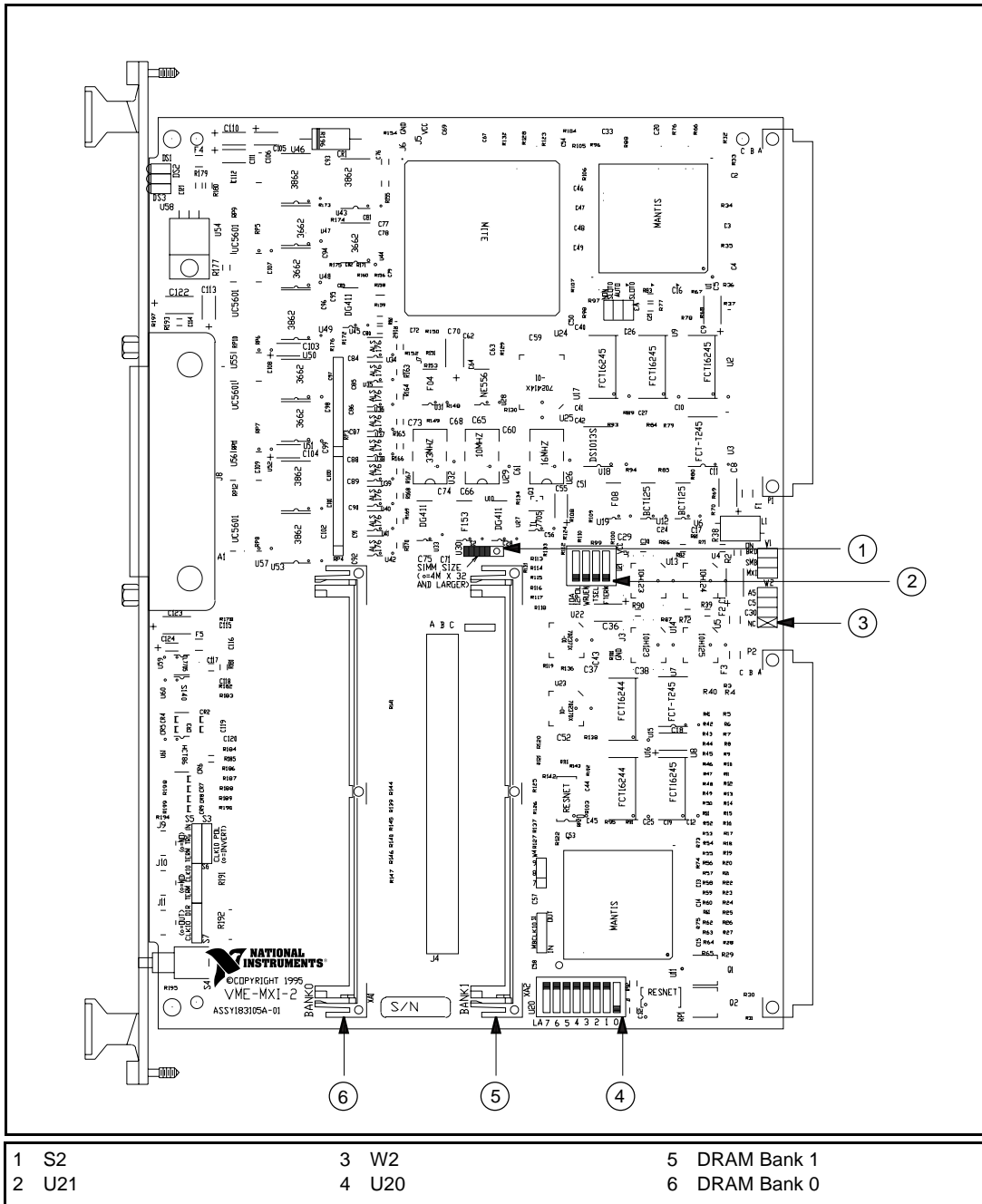
Figure 6-1. VME-MXI-2 Parts Locator Diagram
