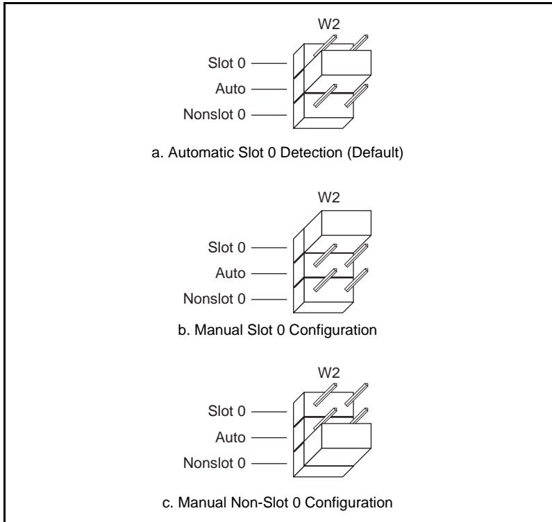
Figure 4-3. VXIbus Slot Configuration
