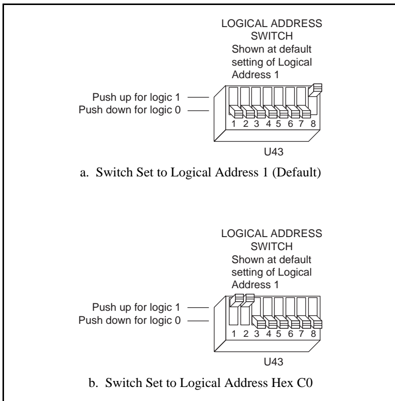
Figure 4-2. Logical Address Selection
