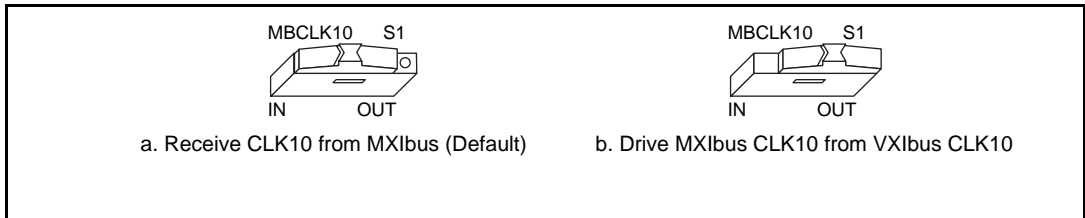
Figure 5-6. Receiving or Driving MXIbus CLK10
