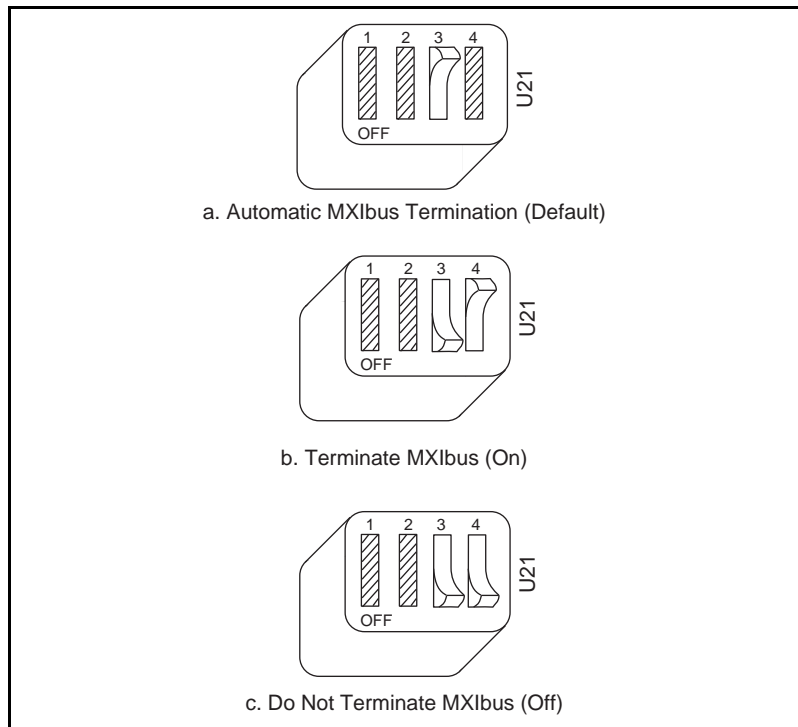
Figure 5-8. MXIbus Termination
