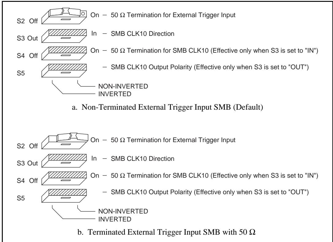
Figure 4-7. SMB Trigger Input Termination
