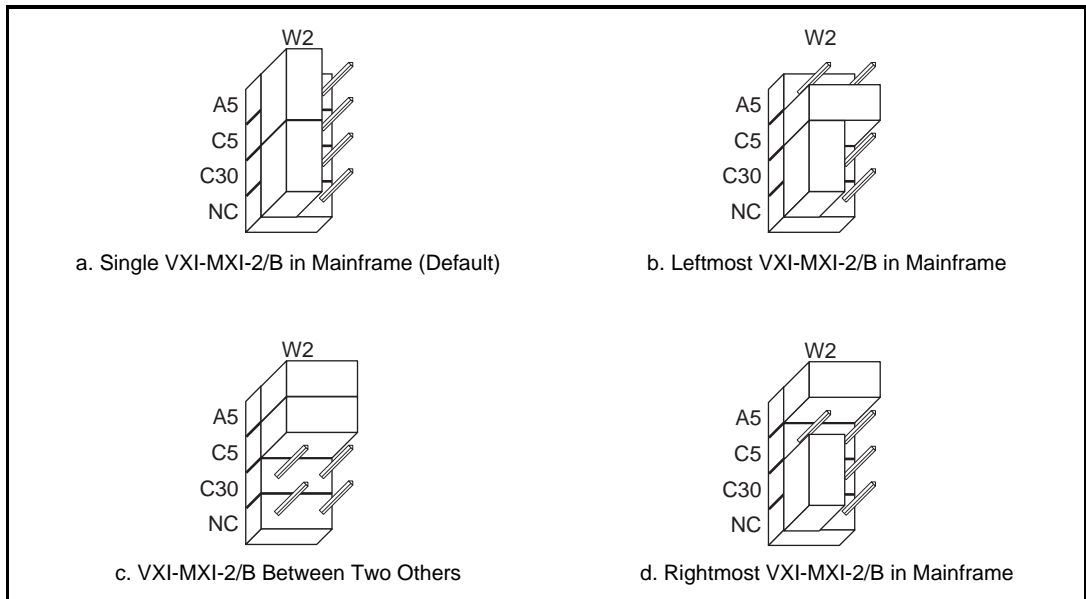
Figure 5-11. VXIbus Local Bus Configuration
