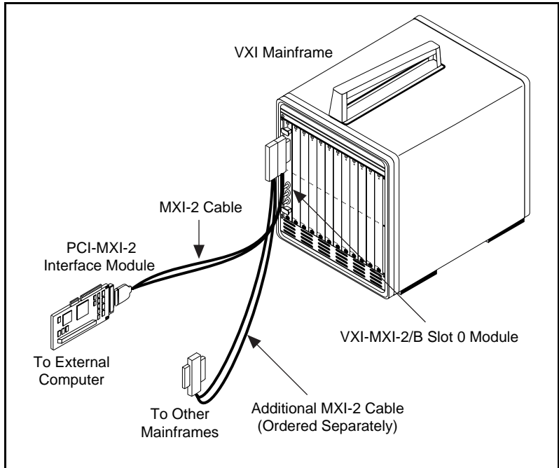
Figure 5-12. MXI-2 Cable Configuration Using a PCI-MXI-2 and a VXI-MXI-2/B
