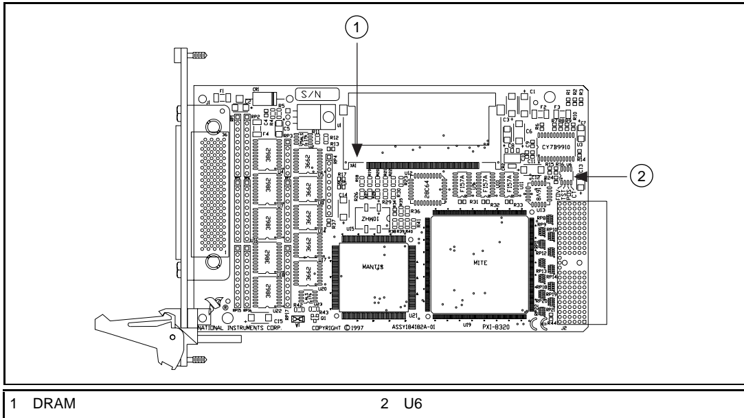
Figure 3-1. PXI-8320 Parts Locator Diagram
