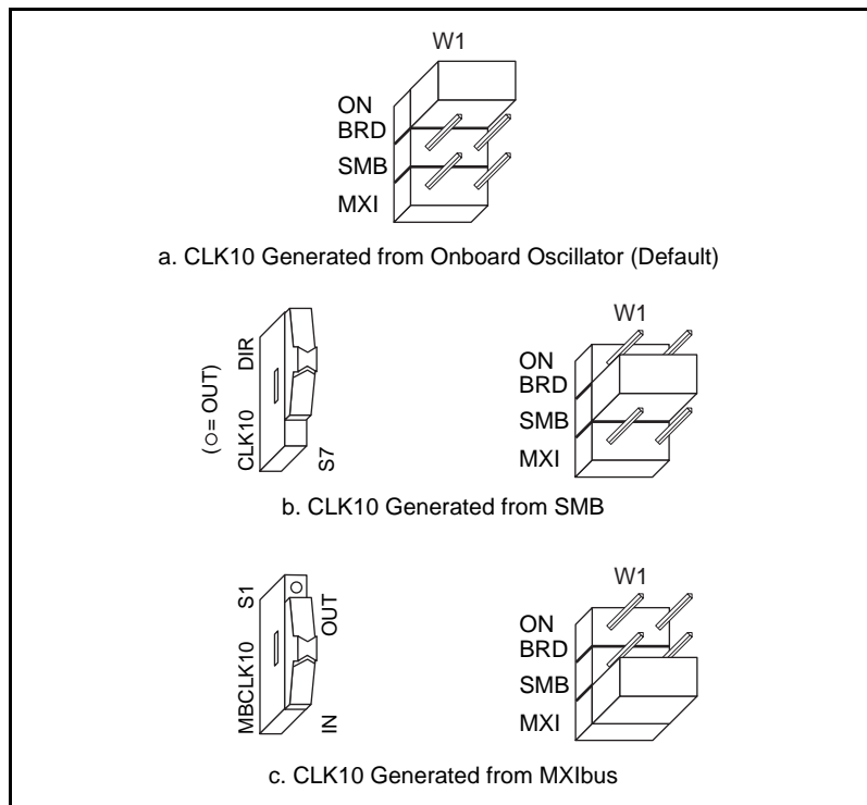
Figure 5-4. VXIbus CLK10 Routing
