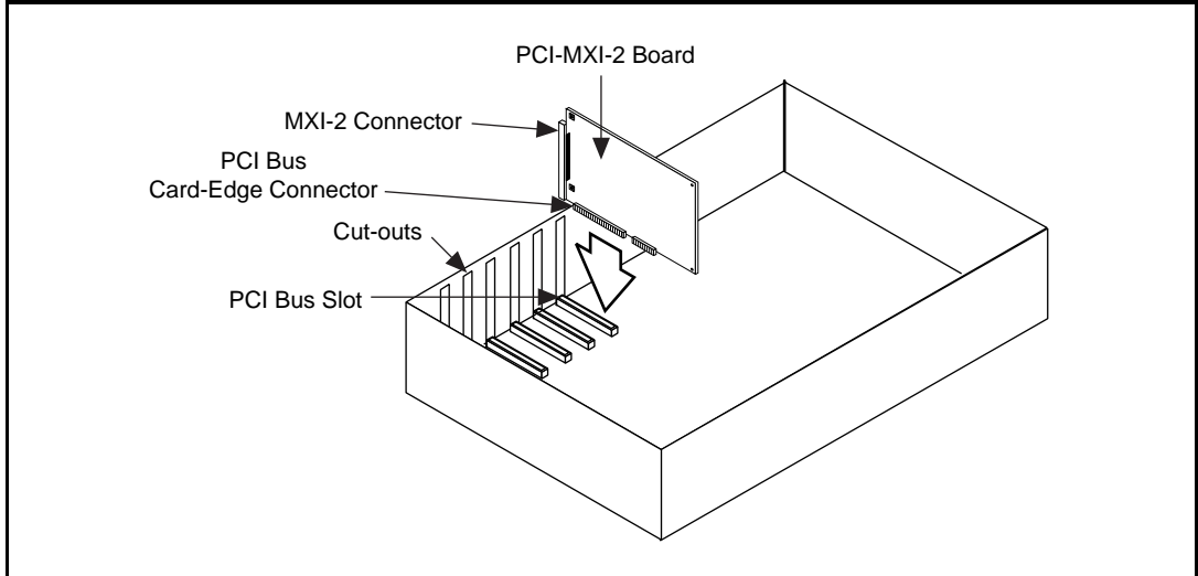
Figure 2-2. Installing the PCI-MXI-2 in a Computer
