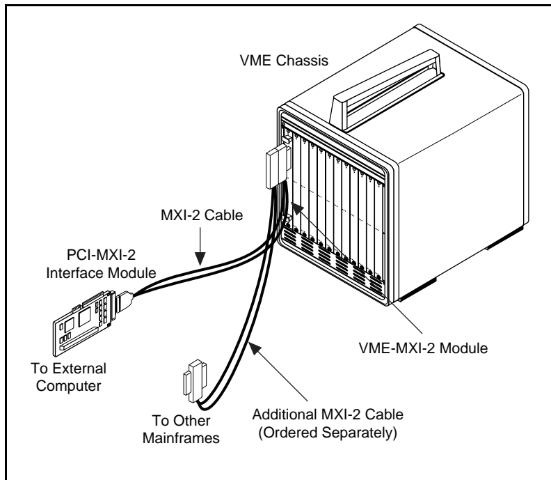
Figure 6-7. MXI-2 Cable Configuration Using a PCI-MXI-2 and a VME-MXI-2
