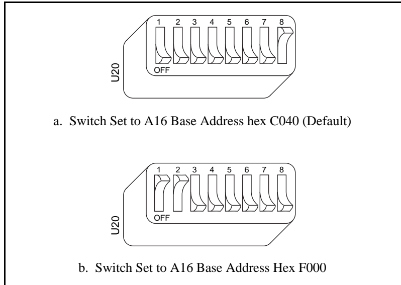
Figure 6-2. Base Address Selection
