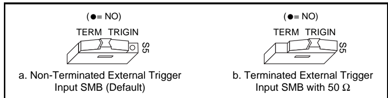
Figure 5-7. SMB Trigger Input Termination
