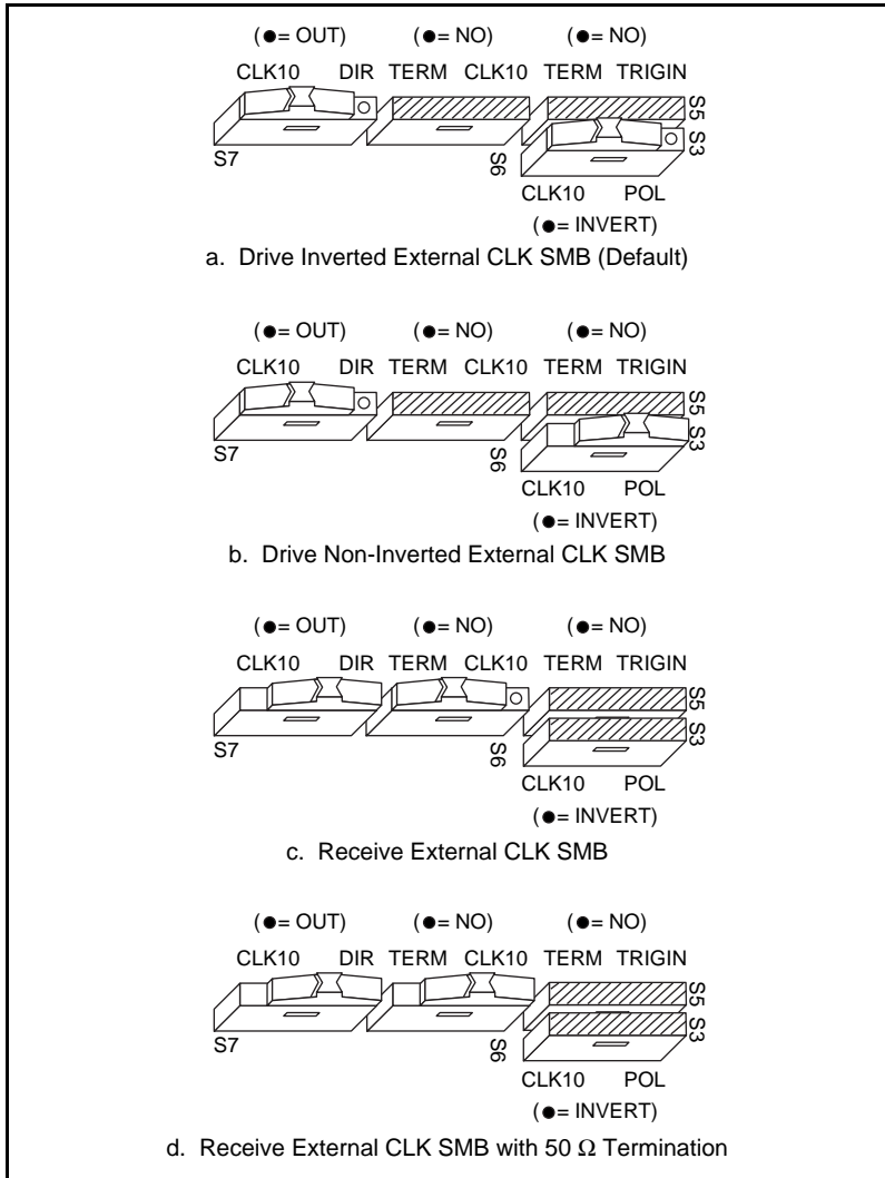
Figure 5-5. SMB CLK10 Settings
