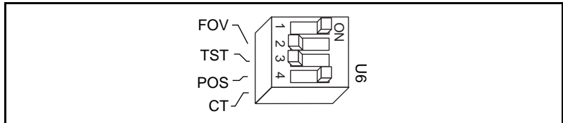
Figure B-4. Restoring the Factory Configuration on the PXI-8320
