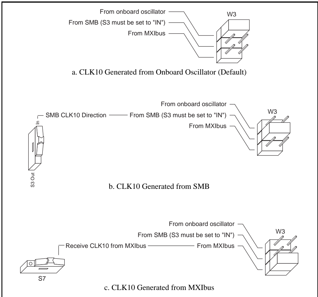
Figure 4-4. VXIbus CLK10 Routing
