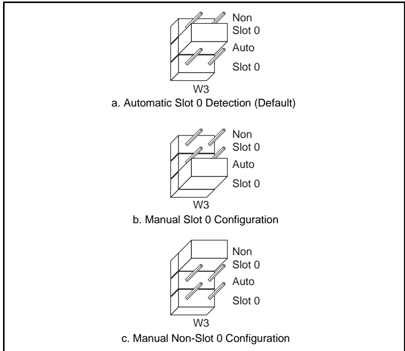
Figure 5-3. VXIbus Slot Configuration
