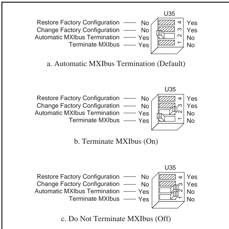
Figure 4-8. MXIbus Termination
