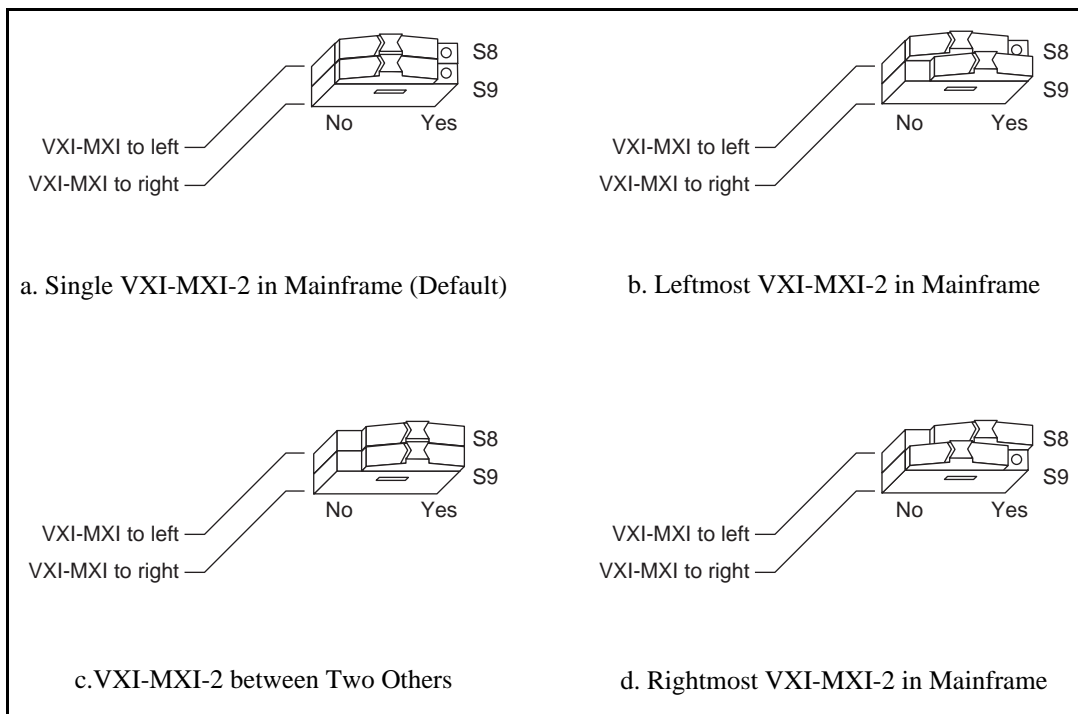
Figure 4-11. VXIbus Local Bus Configuration
