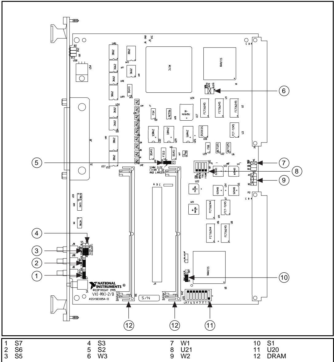
Figure 5-1. VXI-MXI-2/B Parts Locator Diagram
