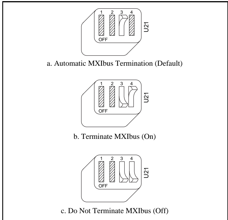
Figure 6-3. MXIbus Termination
