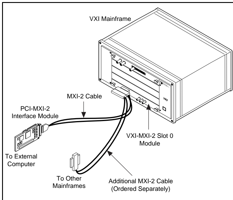
Figure 4-12. MXI-2 Cable Configuration Using a PCI-MXI-2 and a VXI-MXI-2
