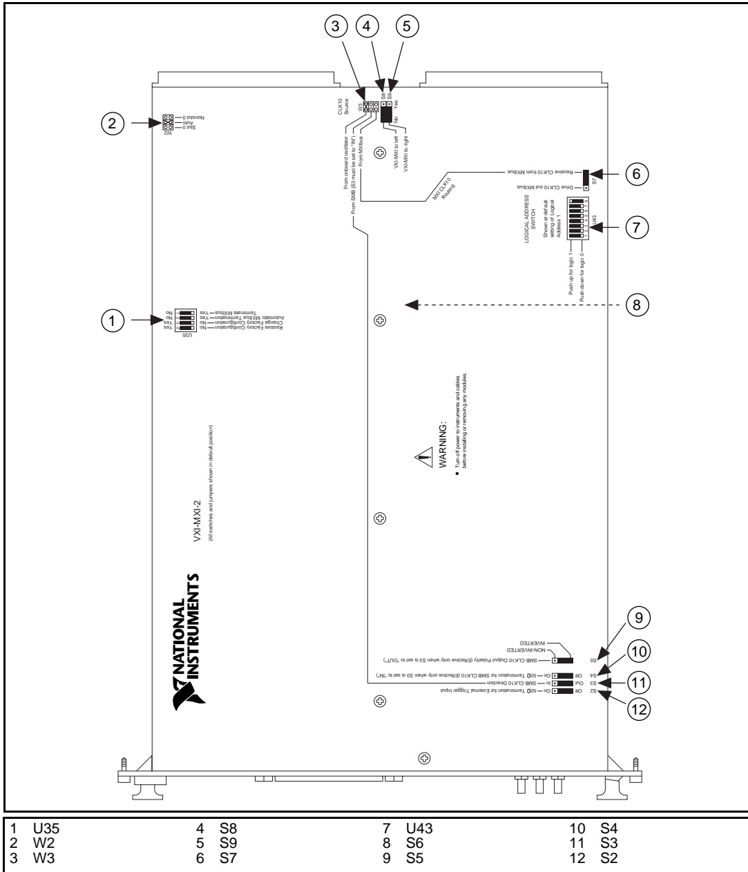
Figure 4-1. VXI-MXI-2 Right-Side Cover
