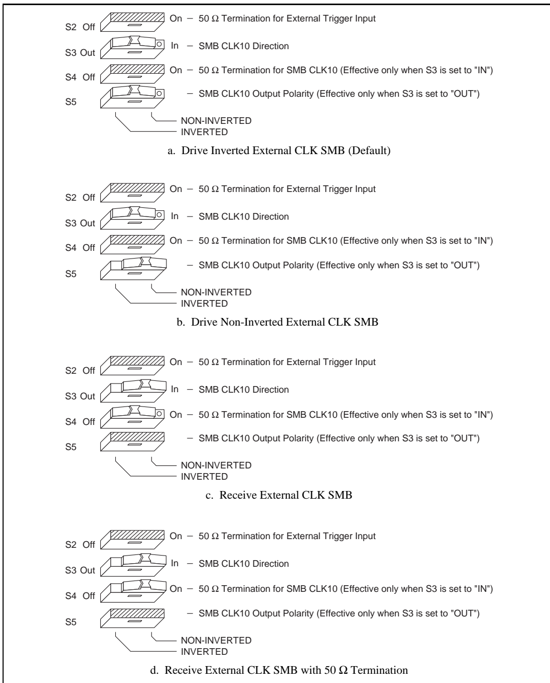
Figure 4-5. SMB CLK10 Settings
