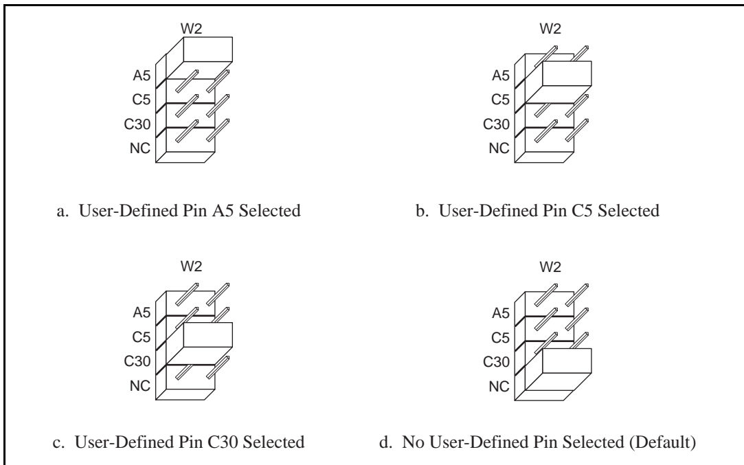
Figure 6-6. VME-MXI-2 Intermodule Signaling Settings
