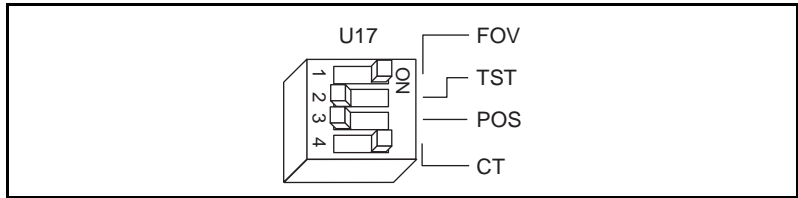
Figure B-3. Restoring the Factory Configuration on the PCI-MXI-2
