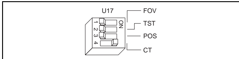
Figure B-1. Normal EEPROM Operation on the PCI-MXI-2
