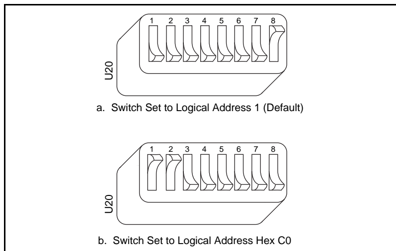
Figure 5-2. Logical Address Selection
