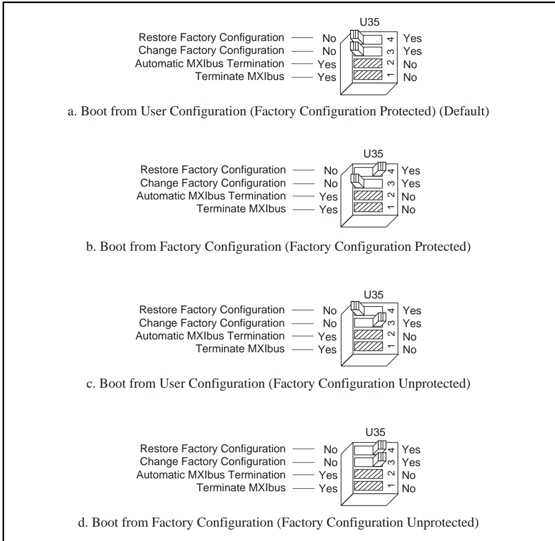
Figure 4-9. EEPROM Operation
